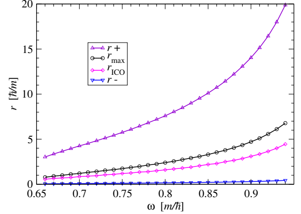
FIG. 16 (color online). Innermost circular orbit radius r_{\text{ICO}} as a function of \omega for boson stars with k = 1 . r_{\text{max}} is the location of the maximum of the scalar field modulus \phi , while r_+ and r_- denote the radii where \phi = \phi_{\text{max}}/10 .
