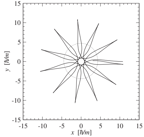
FIG. 23. Same as Fig. 22 but for k = 2 .
