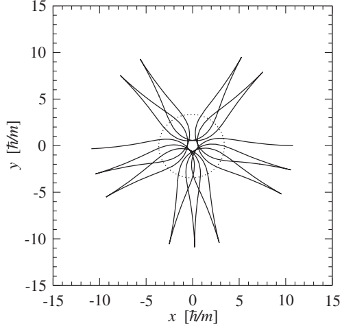
FIG. 25. Same as Fig. 23 but for \omega = 0.75 m/\hbar .
