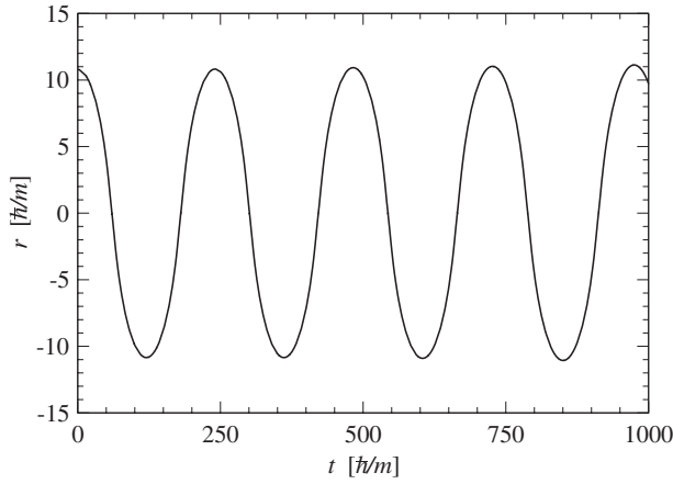
FIG. 21. Evolution of the r coordinate of an \ell = 0 test particle initially at rest at r_i = 10.79\hbar/m in the spacetime generated by a spherical ( k = 0 ) boson star with \omega = 0.77 m/\hbar .
