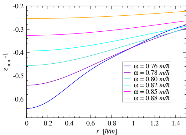
FIG. 18 (color online). Effective potentials for \ell = 0 and for spherical boson stars with different values of \omega (decreasing from top to bottom).
