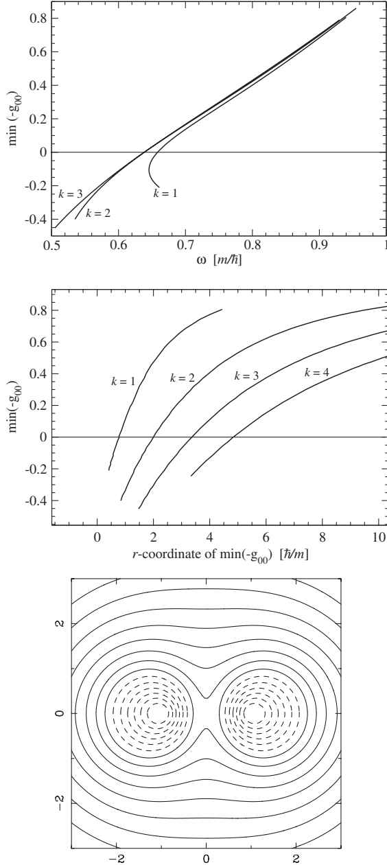
FIG. 10. The first and second panels show the value of the minimum of -g_{00} for free-field boson stars of different rotational quantum number k , as a function of \omega and the location of the minimum, respectively. Isocontours of -g_{00} in a plane of constant (t, \varphi) are plotted in the third panel, for k = 2 and \omega = 0.55m/\hbar . The Cartesian-like coordinates of this plot are x := r \sin \theta and z := r \cos \theta , in units of \hbar/m . The ergoregion is the torus shown in dashed lines.
