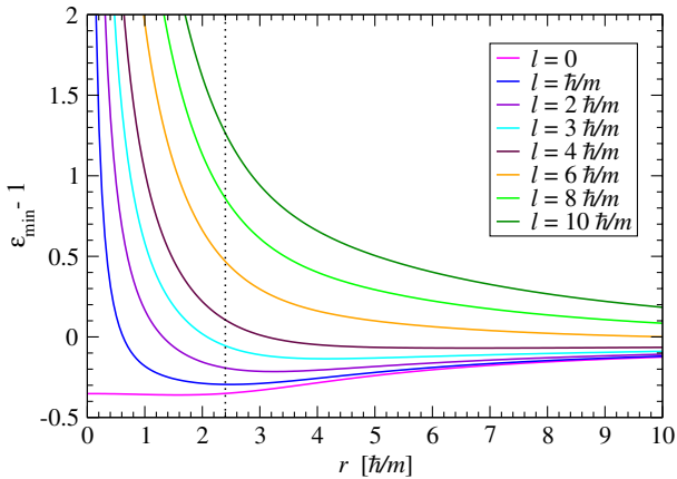
FIG. 13 (color online). Effective potential profiles for a free-field rotating boson star with \omega = 0.8 m/\hbar and k = 1 . The vertical line represents the location of the maximum of the scalar field modulus \phi (cf. Fig. 8).
