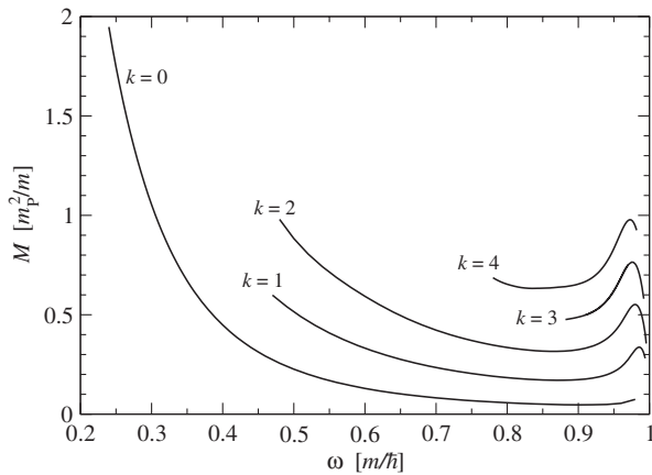
FIG. 12. Gravitational mass as a function of \omega for boson star models constructed upon the self-interacting potential (6) with \sigma = 0.05 , with different values of the rotational quantum number k .
