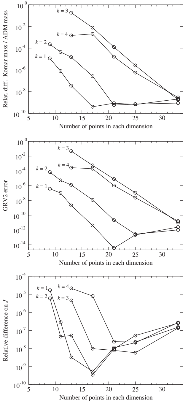
FIG. 5. Various error indicators as the number of spectral coefficients in both the radial and angular dimensions, for free scalar field configurations with \omega = 0.8m/\hbar and rotational quantum number k = 1, 2, 3 and 4. The first panel shows the error on the masses, the second one on the GRV2 identity and the last one on the angular momentum.
