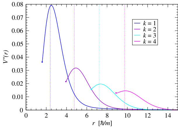
FIG. 17 (color online). \mathcal{V}''(r) for rotating boson stars with \omega = 0.8 m/\hbar . We choose \varepsilon = 4.2 and \ell = 1.2\hbar/m . The vertical lines mark the position of the maximum of the scalar field modulus for each boson star.
