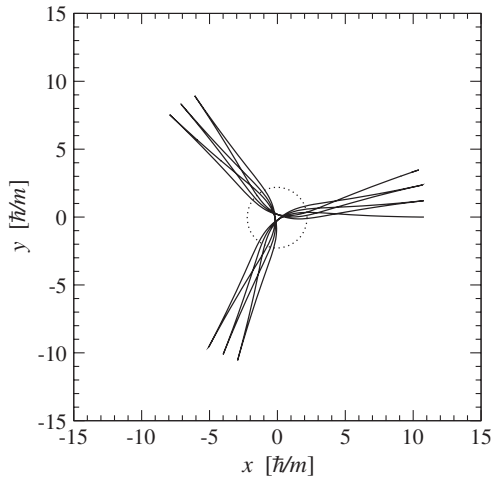
FIG. 22. Orbit of an \ell = 0 test particle in the equatorial plane of a rotating free-field boson star with k = 1 and \omega = 0.80 m/\hbar ; the particle is initially at rest at r = r_i = 10.79\hbar/m and \varphi = 0 . The Cartesian-like coordinates of the plot are x := r \cos \varphi and y := r \sin \varphi . The dotted circle marks the maximum of the scalar field modulus \phi .
