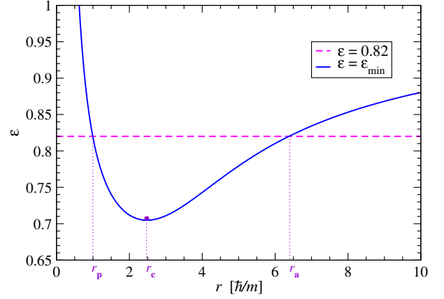
FIG. 14 (color online). Effective potential profile for \ell = 1\hbar/m . Only the region where \varepsilon \geq \varepsilon_{\text{min}} is allowed for the motion of the test particle, so the radial coordinate r must obey r_p \leq r \leq r_a . The spot marks the position of the stable circular orbit of radius r_c .
