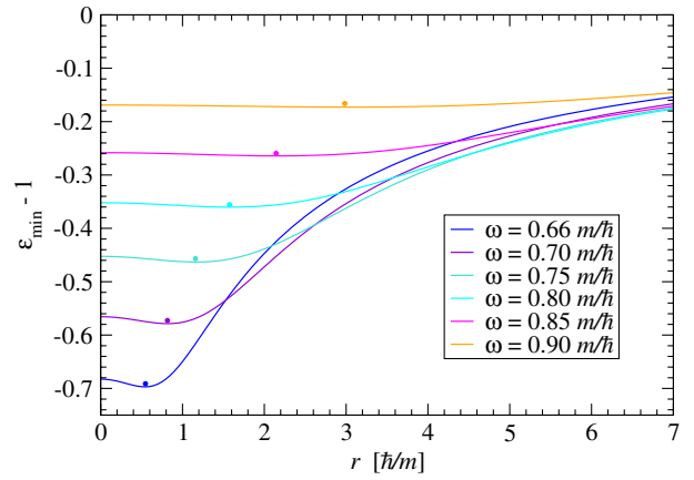
FIG. 19 (color online). Effective potential for \ell = 0 and for rotating boson stars with k=1 and different values of \omega (decreasing from top to bottom). The dots mark the position of the stable circular orbits.
