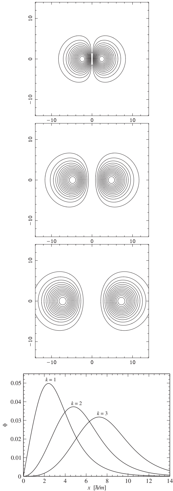
FIG. 8. Isocontours of the scalar field modulus \phi in a meridian plane of constant (t, \varphi) for \omega = 0.8m/\hbar in all plots and k = 1 (first panel), k = 2 (second one) and k = 3 (third one). The Cartesian-like coordinates used for the plot are x := r \sin \theta (horizontal axis) and z := r \cos \theta (vertical axis), in units of \hbar/m . The fourth panel shows, for the same configurations, the profiles of \phi along the x -axis, i.e. the functions \phi(r, \pi/2) .
