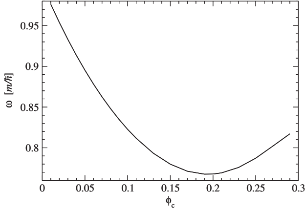
FIG. 2. Value of \omega as a function of \phi_c for spherical configurations and a free scalar field.
