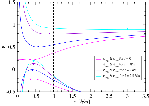
FIG. 15 (color online). Effective potential profiles for the free-field rotating boson star with \omega = 0.646 m/\hbar and k = 1 . The ergoregion is delimited by the vertical dot-dashed and dashed lines; the thin vertical dotted line marks the maximum of the scalar field modulus \phi . The plots for \varepsilon \geq 0.2 are those of \varepsilon_{\min} , while the plots for \varepsilon \leq 0.2 are those of \varepsilon_{\text{neg}} . The latter ones can be used to determine orbits only inside the ergoregion. There is a circular stable orbit (marked with a dot) for each minimum of \varepsilon_{\min} and for each maximum of \varepsilon_{\text{neg}} .
