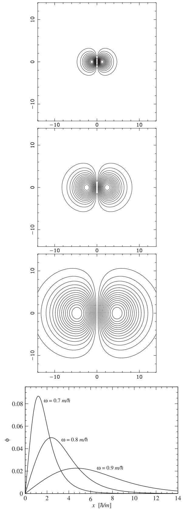
FIG. 9. Same as Fig. 8 but for k = 1 in all plots and \omega = 0.7m/\hbar (first panel), \omega = 0.8m/\hbar (second one) and \omega = 0.9m/\hbar (third one).
