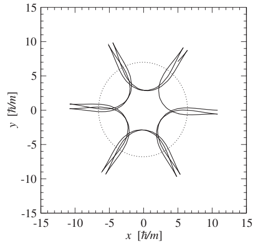
FIG. 24. Same as Fig. 22 but for k = 3 .
