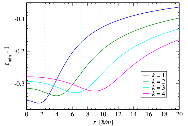
FIG. 20 (color online). Effective potential for \ell = 0 and for rotating boson stars with \omega = 0.8 m/\hbar and different values of k . The vertical lines mark the position of the maximum of the scalar field modulus for each boson star.
