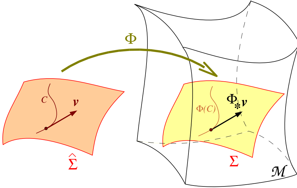
Figure 2.1: Embedding \Phi of the 3-dimensional manifold \hat{\Sigma} into the 4-dimensional manifold \mathcal{M} , defining the hypersurface \Sigma = \Phi(\hat{\Sigma}) . The push-forward \Phi_*v of a vector v tangent to some curve C in \hat{\Sigma} is a vector tangent to \Phi(C) in \mathcal{M} .
