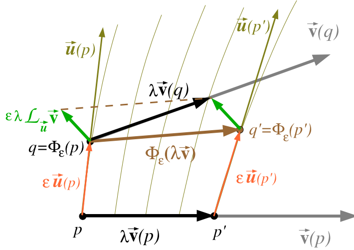
Figure A.1: Geometrical construction of the Lie derivative of a vector field: given a small parameter \lambda , each extremity of the arrow \lambda \mathbf{v} is dragged by some small parameter \varepsilon along \mathbf{u} , to form the vector denoted by \Phi_\varepsilon(\lambda \mathbf{v}) . The latter is then compared with the actual value of \lambda \mathbf{v} at the point q , the difference (divided by \lambda \varepsilon ) defining the Lie derivative \mathcal{L}_\mathbf{u} \mathbf{v} .
