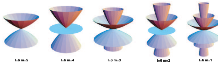
Figure 12: Example of morphologies predicted from solution of a macroscopic Schrödinger equation that describes an accretion or ejection process. This problem is similar to that of scattering in elementary particle physics (spherical ingoing or outgoing wave). Such morphologies are typical of those observed in 'planetary nebula', which are, despite their names, stars that eject their outer shells (see [56]).
