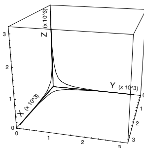
Figure 7: ‘Three-tip string’. Three dimensional sphere in scale space, (\ln X)^2 + (\ln Y)^2 + (\ln Z)^2 = A^2 , plotted in terms of direct variables (X, Y, Z) , for A = 8 .
