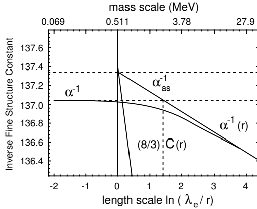
Figure 18: Observed convergence at the electron mass-scale (i.e. at the Compton length of the electron) of the asymptotic running electromagnetic inverse coupling \alpha^{-1}(r) and of the running scale-relativity constant 8\mathcal{T}(r)/3 = 8 \ln[m_P/m(r)] . Such a convergence is theoretically expected in the framework of the scale-relativistic interpretation of gauge transformations, that yields a mass-charge relation for the electron, that reads 8\alpha_e \ln(m_P/m_e) = 1 . The final low energy fine structure constant differs from its asymptotic value by a small threshold effect (see e.g. [84], [4] Sec.6.2)
