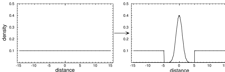
Figure 15: Model of formation of a structure from a background medium. The global harmonic oscillator potential defined by the background induces the formation of a local structure (see a 3D representation in Fig. 16), in such a way that the average density remains constant (i.e., the matter of the structure is taken from the medium).
