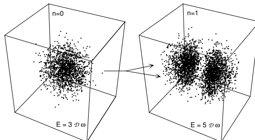
Figure 16: Model of duplication. The stationary solutions of the Schrödinger equation in a 3D harmonic oscillator potential can take only discretized morphologies in correspondence with the quantized value of the energy. Provided the energy increases from the one-object case ( E_0 = 3D\omega ), no stable solution can exist before it reaches the second quantized level at E_1 = 5D\omega . The solutions of the time-dependent equation show that the system jumps from the one object to the two-object morphology.
