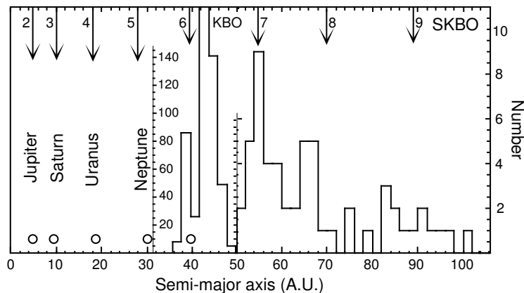
Figure 9: Distribution of the semi-major axis of Kuiper belt objects (KBO) and scattered Kuiper belt objects (SKBO), compared with the theoretical predictions of probability density peaks for the outer solar system (arrows) [56]. The whole inner solar system (whose density peak lies at the Earth distance, that corresponds to n_i = 5 ) can be identified with the fundamental n_e = 1 orbital of the outer solar system [51]. Therefore the outer solar system is expected to be organized according to a constant w_e = 144/5 = 28.8 km/s. Remark that the existence of probability density peaks for the Kuiper belt small planets at \approx 40, 55, 70, 90 AU, etc..., has been theoretically predicted before the discovery of these objects [62].
