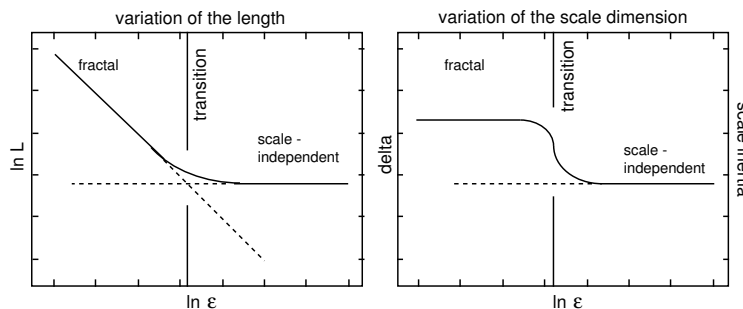
Figure 1: Scale dependence of the length and of the effective scale-dimension in the case of ‘inertial’ scale laws (which are solutions of the simplest, first order scale-differential equation): toward the small scale one gets a scale-invariant law with constant fractal dimension, while the explicit scale-dependence is lost at scales larger than some transition scale \lambda .
