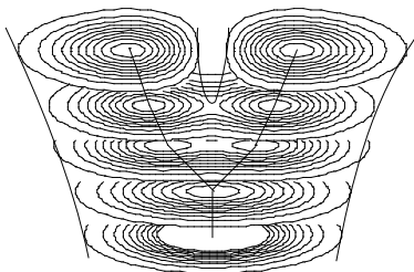
Figure 17: Model of branching / bifurcation. Successive solutions of the time-dependent 2D Schrödinger equation in an harmonic oscillator potential are plotted as isodensities. The energy varies from the fundamental level ( n = 0 ) to the first excited level ( n = 1 ), and as a consequence the system jumps from a one-object to a two-object morphology.
