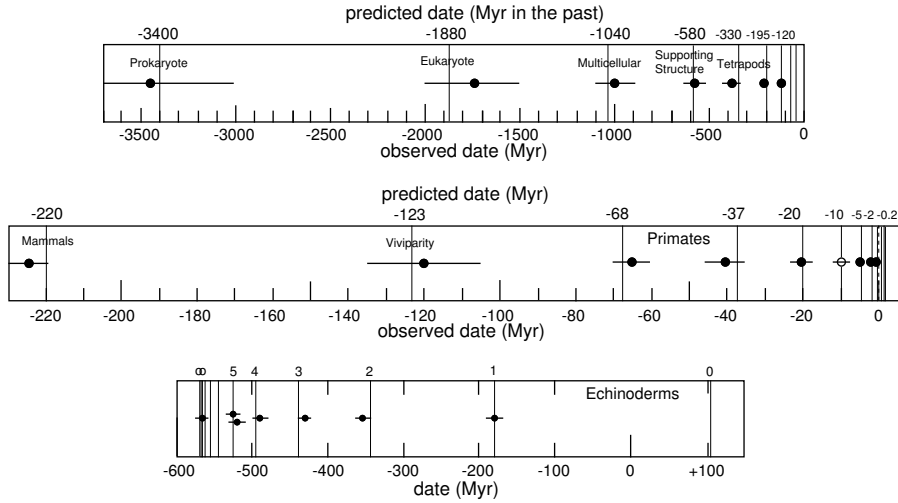
Figure 4: Three typical examples of log-periodic chronological laws in species evolution (from Refs.[40, 41, 42]). Up : main trunk of the ‘tree of life’, from the apparition of life to homeothermy and viviparity (last two plotted points). The dates are best-fitted by an accelerating log-periodic law T_n = T_0 + (T_c - T_0) \times g^{-n} , with T_c = -30 \pm 60 Myr and g = 1.83 . Middle : comparison of the dates of the major leaps in the evolution of primates including the hominids (plus the two preceding main events: apparition of mammals and viviparity), with an accelerating log-periodic law. The best fit gives T_c = 2.0 \pm 0.4 Myr and g = 1.78 \pm 0.01 . For the 14 dates from the origin of life to the appearance of the Homo sapiens bauplan, one finds T_c = 2.1 \pm 1.0 Myr and g = 1.76 \pm 0.01 . The probability is less than 10^{-4} to obtain such a fit by chance. Down : comparison with a decelerating log-periodic law of the dates of the major leaps in the evolution of echinoderms. The best fit yields T_c = -575 \pm 25 Myr and g = 1.67 \pm 0.02 (origin excluded). This means that the critical time from which the deceleration starts is their date of apparition (within uncertainties). All results are statistically highly significant (see the quoted references for details about the data and their analysis).
