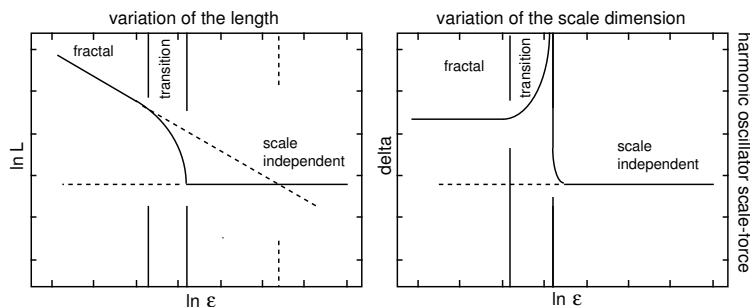
Figure 6: Scale dependence of the length and of the scale dimension in the case of a harmonic oscillator scale-potential.
