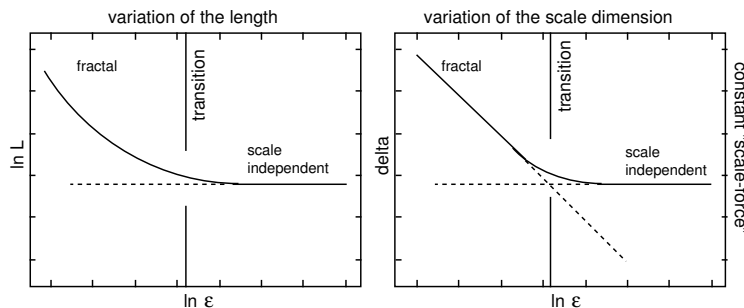
Figure 5: Scale dependence of the length and of the effective scale-dimension in the case of a constant ‘scale-force’.
