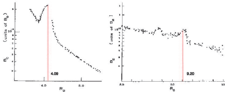
Figure 8: IR-dust density observed during the solar eclipse of January 1967 (adapted from MacQueen [61]). The scale-relativity approach leads to a hierarchical description of the Solar System, which is described by imbricated sub-systems that are solutions of gravitational Schrödinger equations. While the inner solar system is organized on a constant w_0 = 144 km/s, we expect the existence of an intramercurial subsystem organized on the basis of a new constant w = 3 \times 144 = 432 km/s. The Sun radius is in precise agreement with the peak of the fundamental level of this sequence: namely, one finds n_\odot = 0.99 with R_\odot = 0.00465 AU, that corresponds to a Keplerian velocity of 437.1 km/s. The next probability density peaks are predicted to lie at distances 4.09 R_\odot , and 9.20 R_\odot = 0.043 AU, which correspond respectively to Keplerian velocities of 432/2 and 432/3 = 144 km/s. Since 1966, there has been several claims of detection during solar eclipses of IR thermal emission peaks from possible circumsolar dust rings which lie precisely at the predicted distances [56]. Several exoplanets have now been also found at similar relative distances a/M from their star (see Fig. 10).
