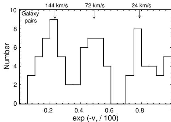
Figure 13: Deprojection of the intervelocity distribution of galaxy pairs [63, 56] from the Schneider-Salpeter catalog with precision redshifts [64]. The main probability peak is found to lie at 144 km/s (plus secondary peaks at 72=144/2 km/s and 24=144/6 km/s), in agreement with the exoplanet and inner solar system structuration (see Fig. 10).
