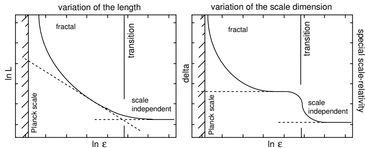
Figure 2: Scale dependence of the length and of the effective scale-dimension in the case of scale-relativistic Lorentzian scale laws.
