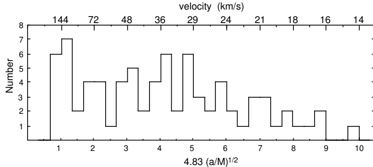
Figure 10: Observed distribution of the semi-major axes of recently discovered exoplanets and inner solar system planets, compared with the theoretical prediction from the scale-relativity / Schrödinger approach. Note that these predictions [4, 62] have been made before the first discovery of exoplanets. One expects the occurrence of peaks of probability density for semimajor axes a_n = GM(n/w_0)^2 , where n is integer, M is the star mass and w_0 = 144.7 \pm 0.7 km/s is a gravitational coupling constant (see [4, 50, 54]). For example, the velocity of Mercury is 48=144/3 km/s, of Venus 36=144/4 km/s, of the Earth 29=144/5 km/s and of Mars 24=144/6 km/s. The data supports the theoretical prediction in a statistically significant way (the probability to obtain such an agreement by chance is P = 4 \times 10^{-5} ).
