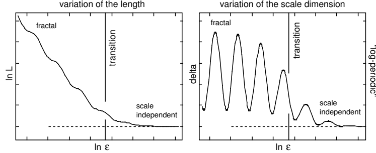
Figure 3: Scale dependence of the length and of the scale dimension in the case of a log-periodic behavior with fractal / nonfractal transition, \mathcal{L}(\varepsilon) = \mathcal{L}_0[1 + (\lambda/\varepsilon)^\nu e^{b \cos(\omega \ln(\varepsilon/\lambda))}] .
