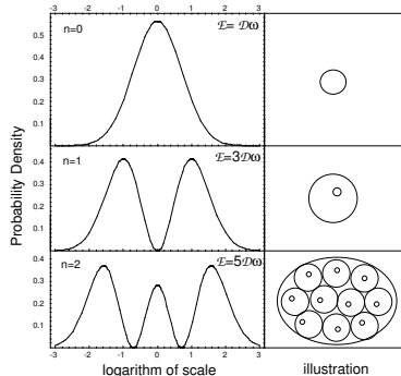
Figure 19: Solutions of increasing complexergy of the scale-Schrödinger equation for an harmonic oscillator scale-potential. These solutions can be interpreted as describing systems characterized by an increasing number of hierarchical levels, as illustrated in the right hand side of the figure. For example, living systems such as procaryots, eucaryots and simple multicellular organisms have respectively one (cell size), two (nucleus and cell) and three (nucleus, cell and organism) characteristic scales.
