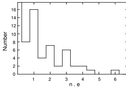
Figure 11: Observed distribution of the eccentricities of exoplanets. The theory predicts that the product of the eccentricity e by the quantity \tilde{n} = 4.83(a/M)^{1/2} , where a is the semi-major axis and M the parent star mass, should cluster around integers. The data support this theoretical prediction at a probability level P = 10^{-4} [60, 56].
